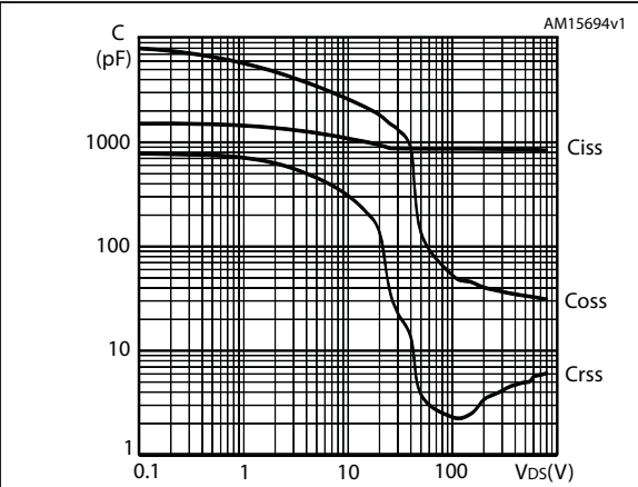
Figure 9. Capacitance variations
