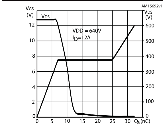
Figure 8. Gate charge vs gate-source voltage
